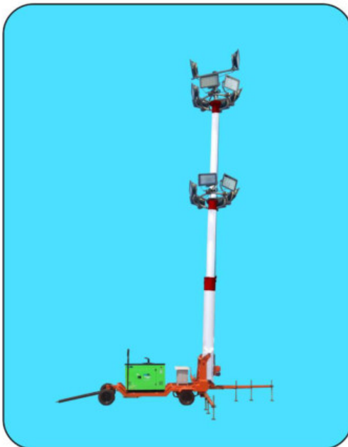
14 / 16 Meter Mobile Lighting Tower
