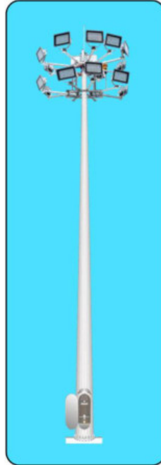
High Mast Lighting System With Double Cradle 12 to 45 Meter
