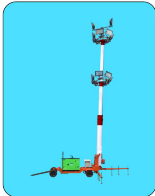
16 / 18 Meter Mobile Lighting Tower
